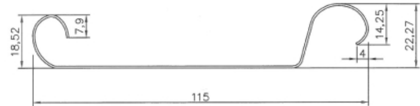
100mm flat insulated lath section
