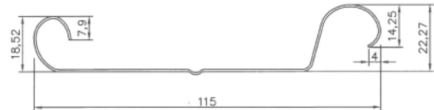
100mm ribbed insulated lath section
